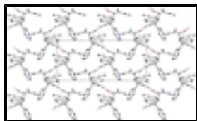
Fig. 2. Packing arrangement of the title compound in the unit cell as viewed down the a axis. The O–H...O and C–H...O intermolecular interactions indicated by dashed lines.
